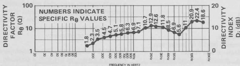
FIGURE 4 — Directivity vs Frequency Whole Space (anechoic)
