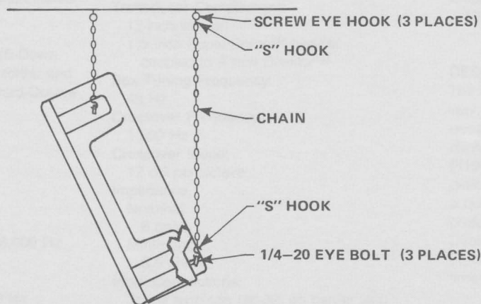
FIGURE 7 – System Mounting
