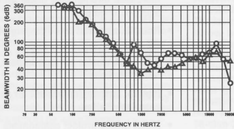
FIGURE 2 — Beamwidth vs. Frequency
