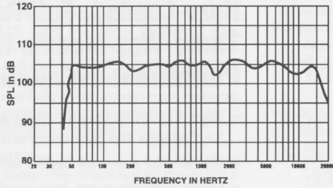
FIGURE 1 — Typical Axial Frequency Response (anechoic environment, 1 watt/1 meter into mid-bass section)
