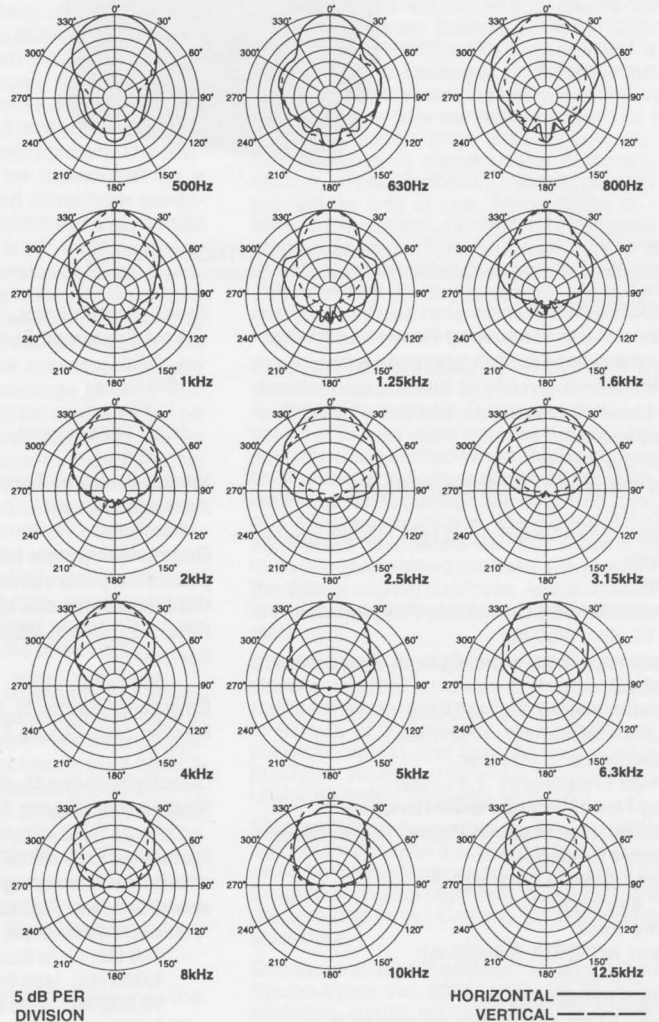
FIGURE 6 — Polar Response
