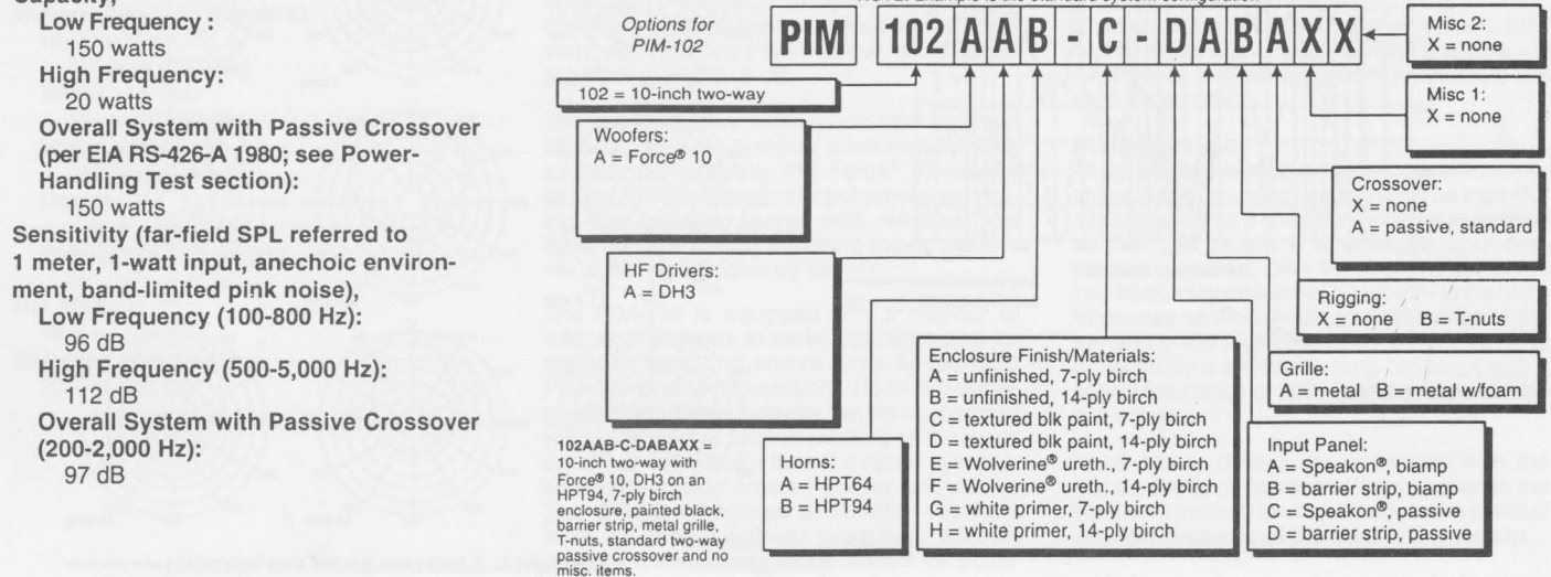
FIGURE 1 — PIM-102 Ordering Matrix
