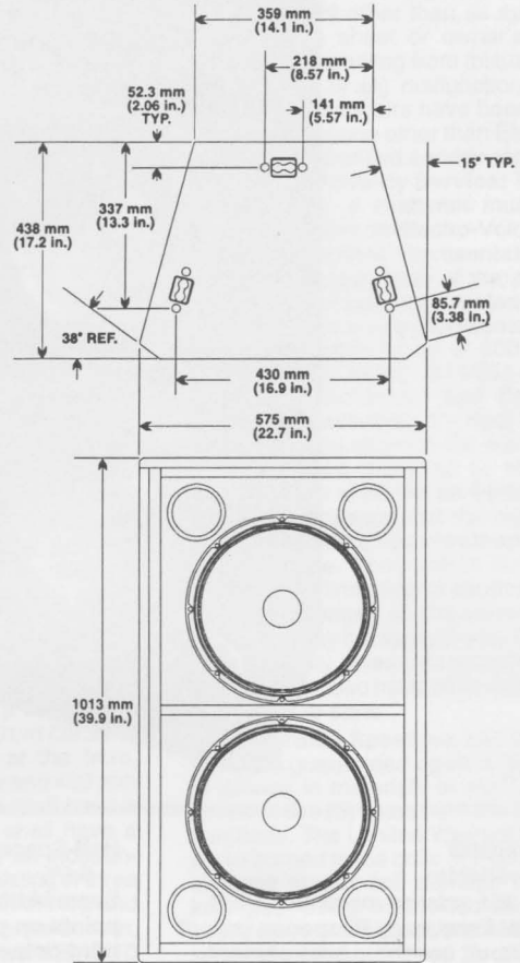
FIGURE 6 — PIM-251 Dimensions
