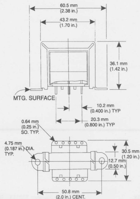
Figure 1 — Dimensions
