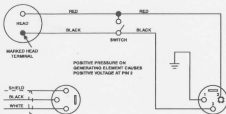
FIGURE 4 Wiring Diagram
