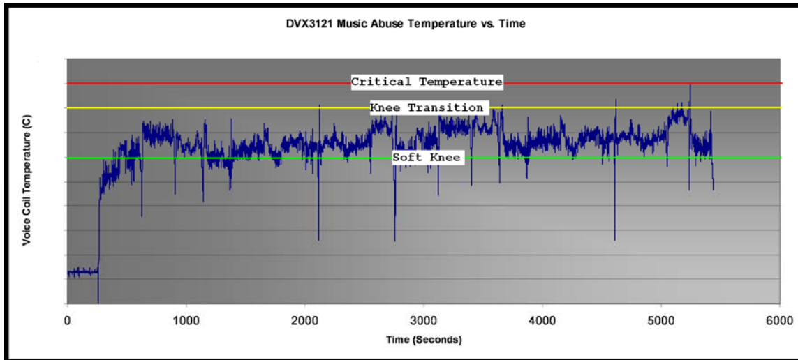
Figure 1: An example of an abusive test with a soft knee at 120C and a critical temperature of 180C.
