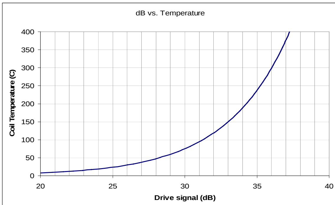
Figure 2: An example of drive level vs. voice coil temperature. The difference between a coil temperature of 250C and 200C is 1dB. This means a 1dB level reduction can prevent component failures!
