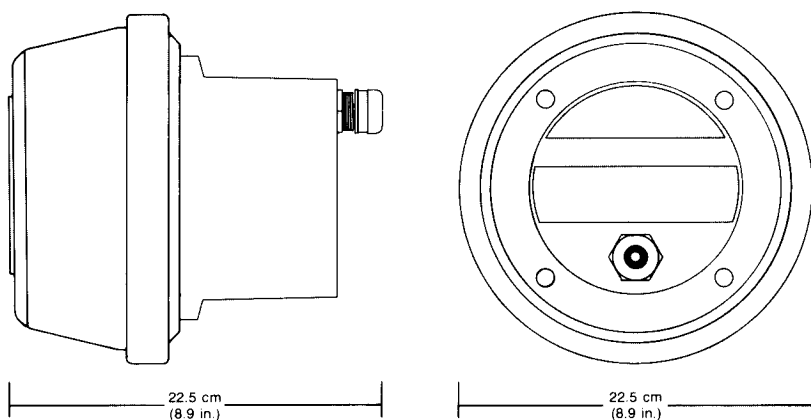
FIGURE 2 — Dimensions
