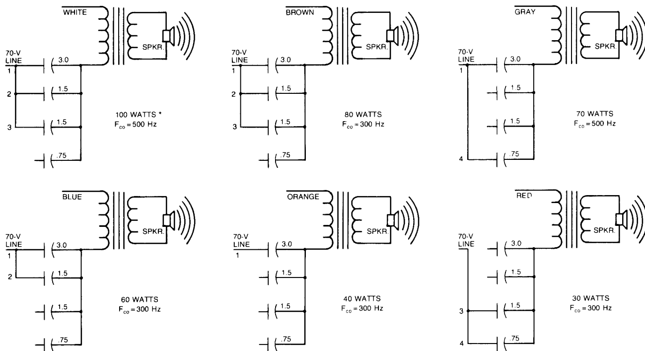
FIGURE 9 — Crossover and Input Options
