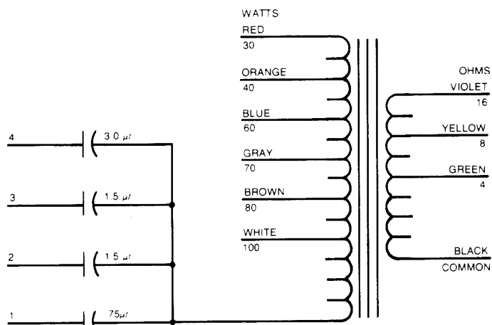
FIGURE 4 — Transformer Schematic
