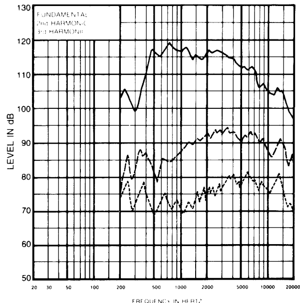
FIGURE 6 — Distortion Response, HP9040 Horn, 5 Watts/1 Meter
