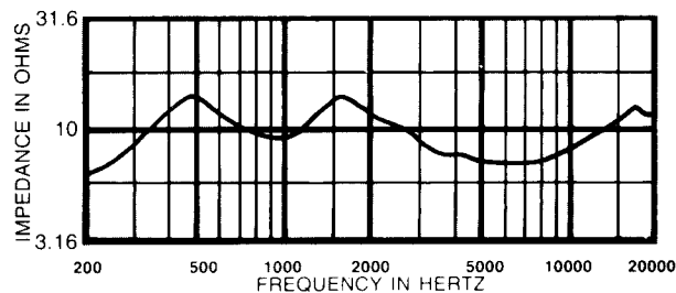
FIGURE 8 — Impedance Response, HP9040 Horn
