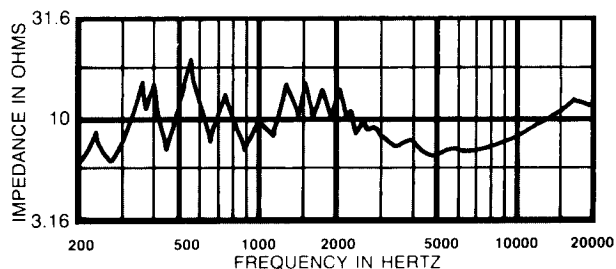
FIGURE 7 — Impedance Response, 2-Inch Plane-Wave Tube
