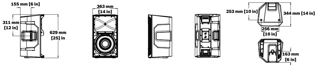
Figure 7.2: Dimensions du ELX200-12
