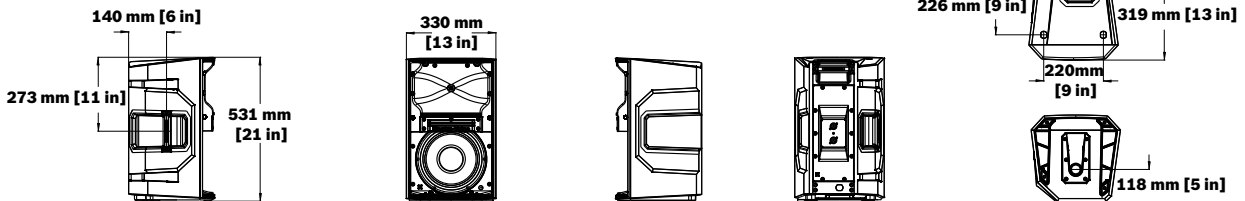
Figure 7.1: Dimensions du ELX200-10
