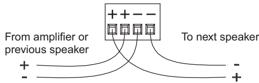
Figure 4.4: Daisy-chain wiring
