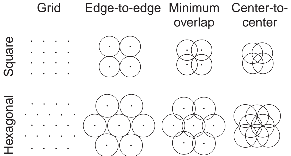
Figure 7.2: Coverage patterns
