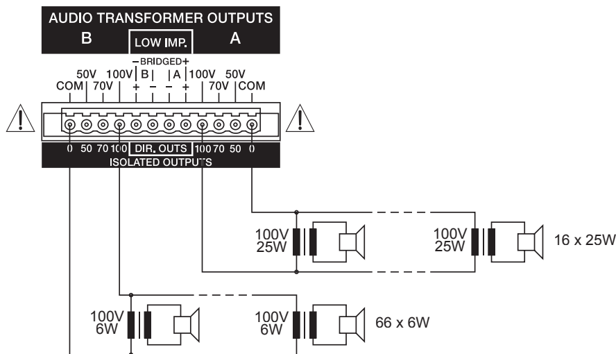
Configuration example: PA2400T with 100V speaker systems connected. Maximum working loads with 25W/100V and 6W/100V loudspeaker systems.
