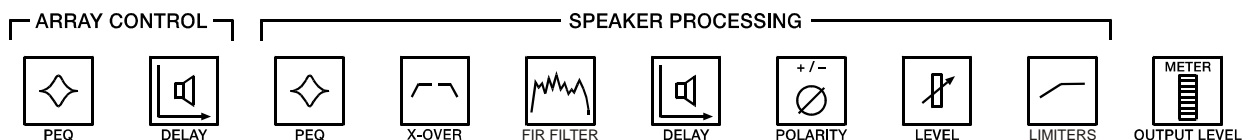
Illustration 5-6: DSP blocks of outputs 1 to 6
