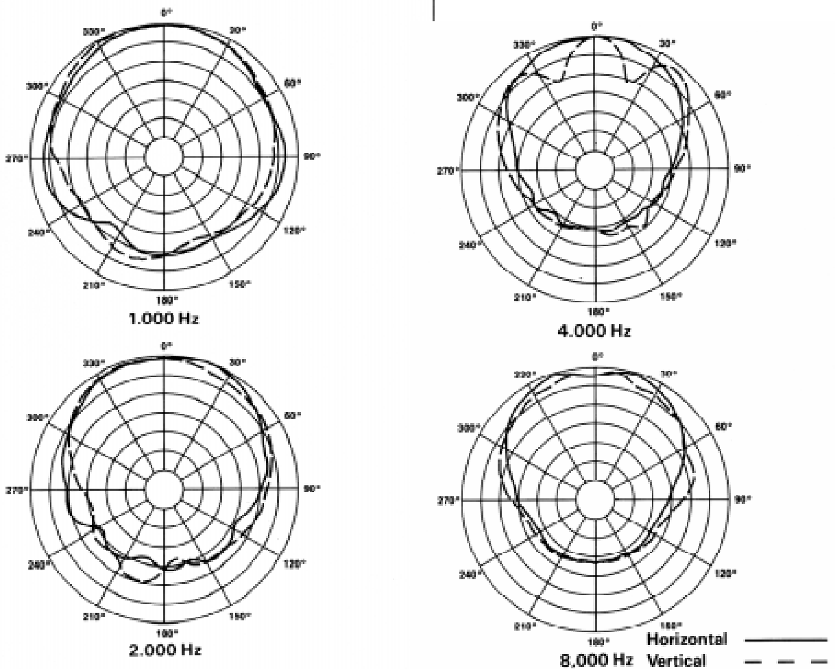
FIGURE-4 Polar Response
