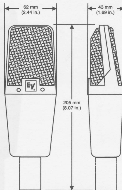
FIGURE 3 — Dimensions
