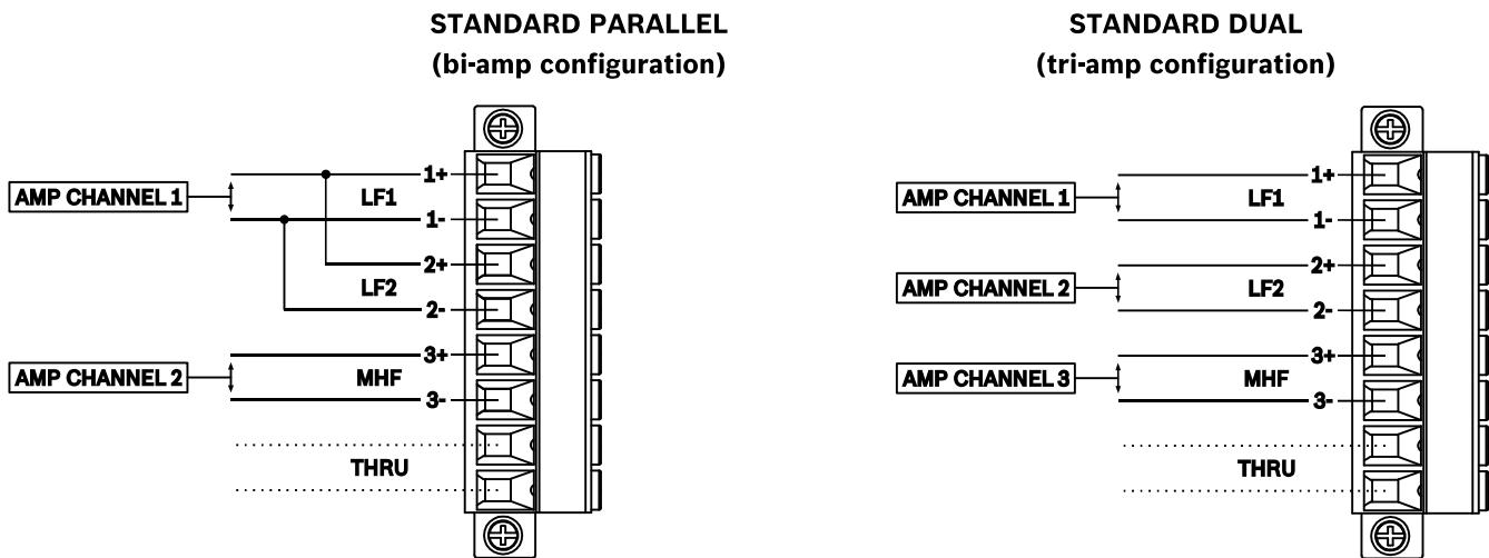
Figure 4.2: Wiring diagrams for standard models
